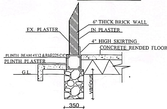
DETAIL OF RUBBLE FOUNDATION
